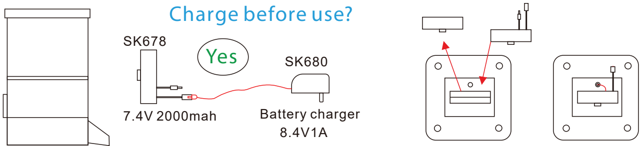
SK670 + rechargeable battery (SK678) + battery charger (SK680)
