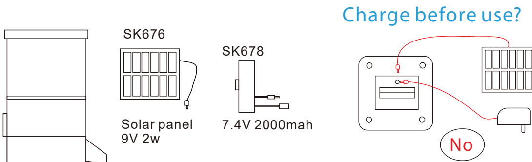
SK670 + Solar Panel (SK676) + rechargeable battery (SK678)
