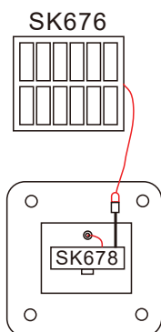
2 Insert battery, connect the wires
